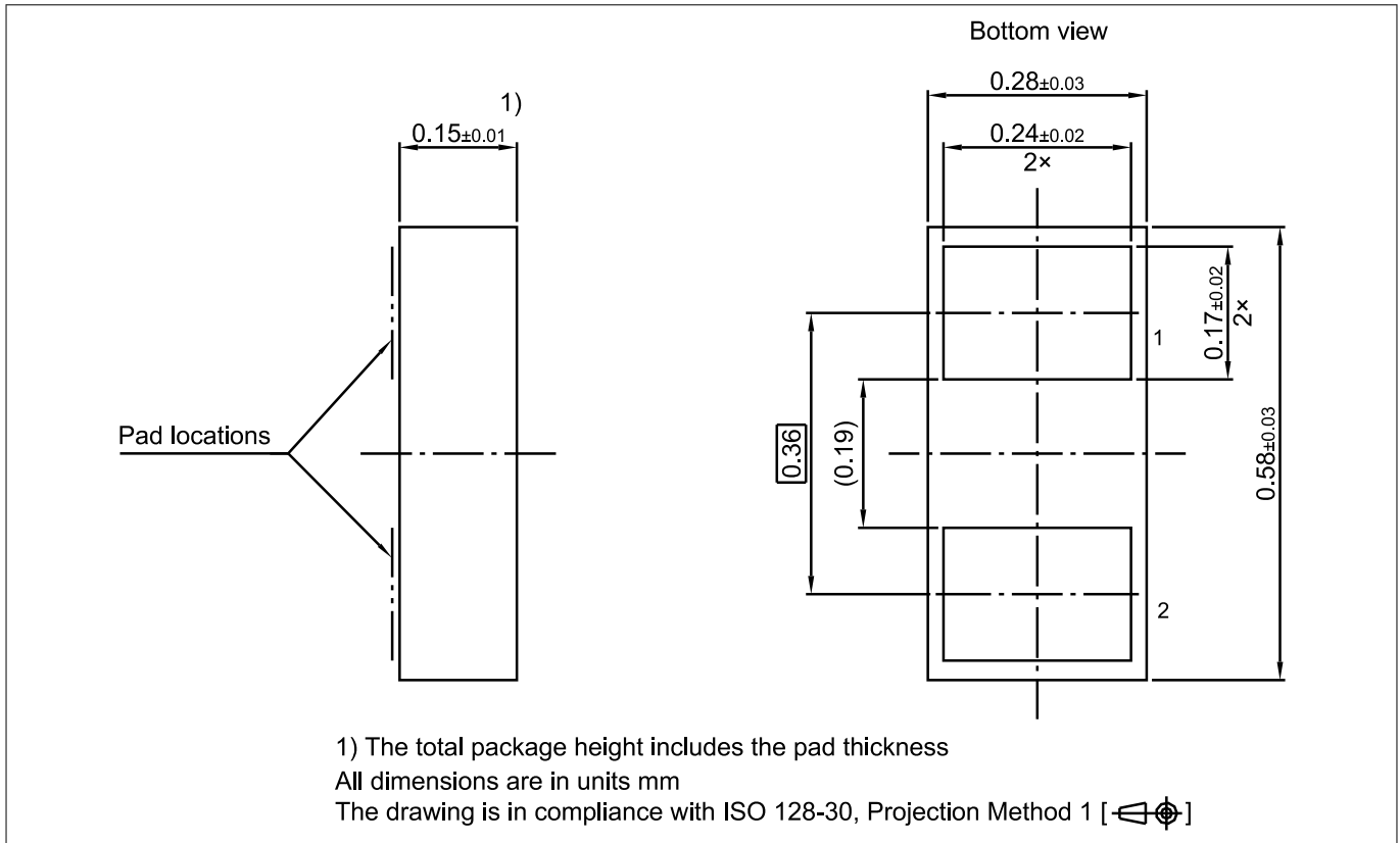
Figure 15 WLL-2-3 package
