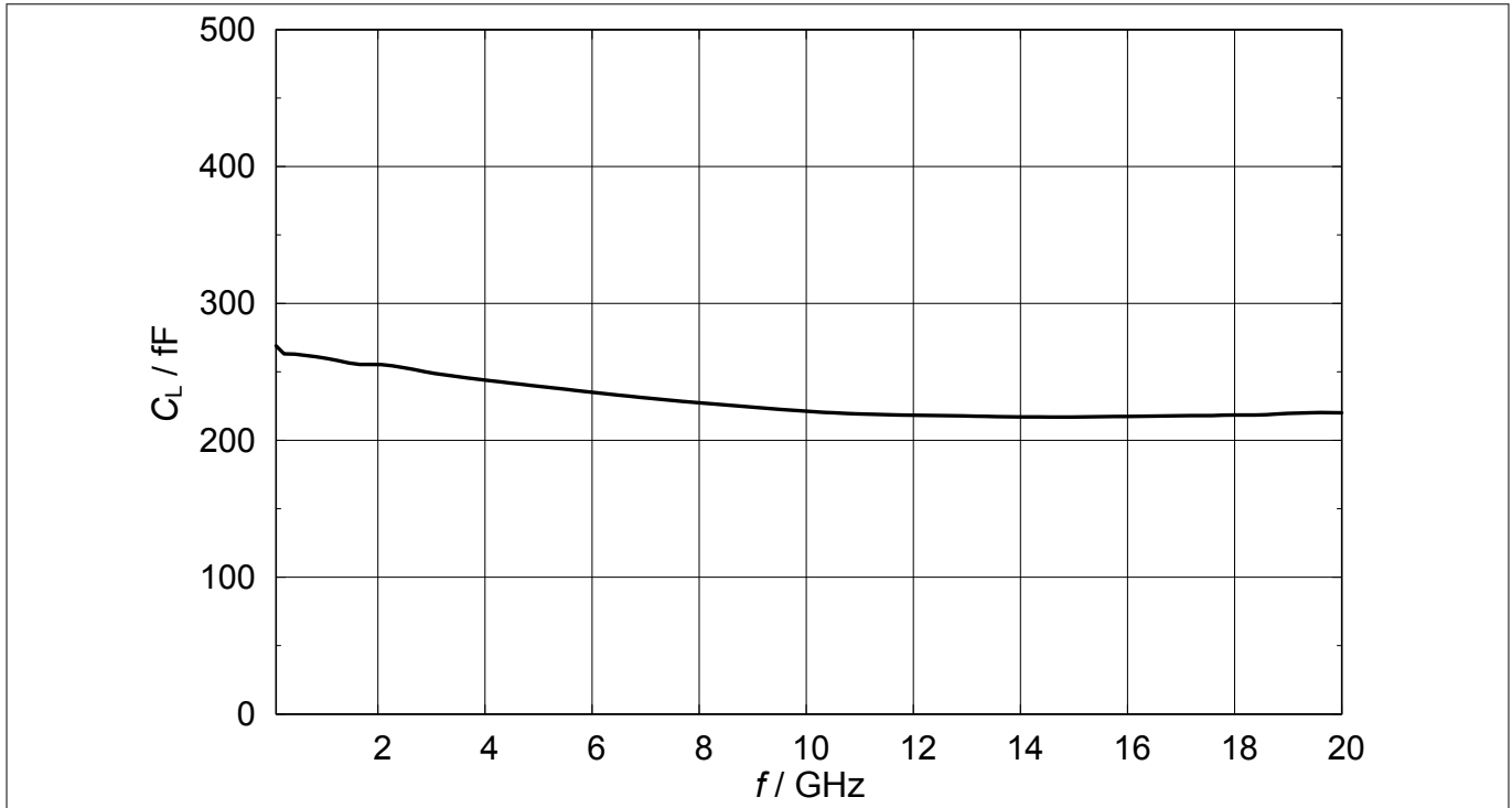
Figure 5 Line capacitance: C_L = f(f) = 1 MHz
